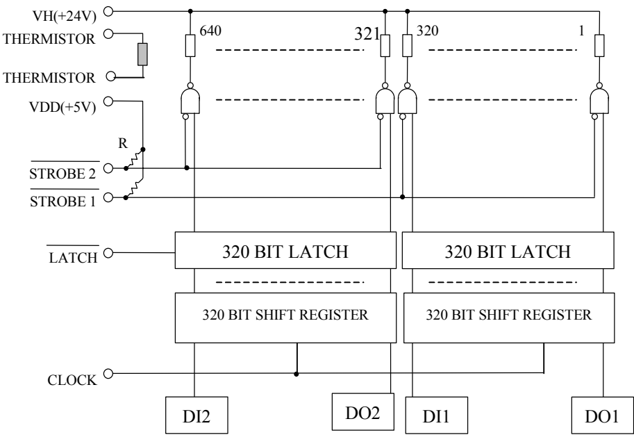
Fig. 3 Schematic Diagram
