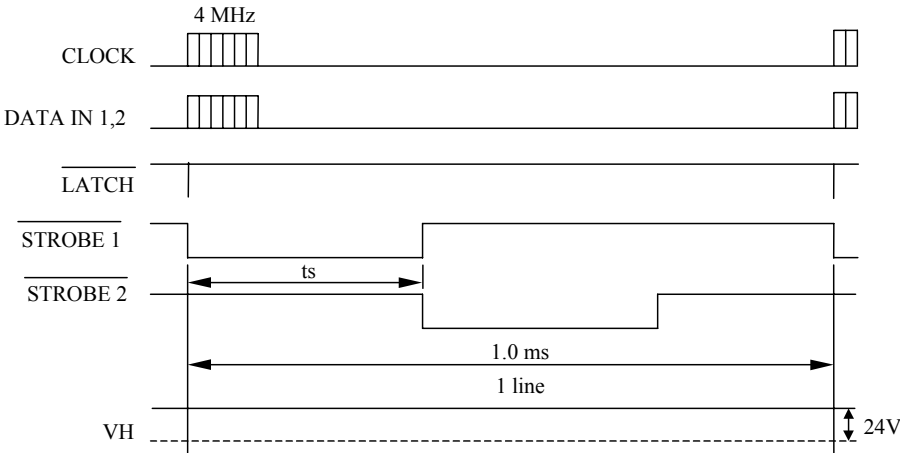
Fig. 2 Thermal Print Head (3T54-2I) Timing Chart
