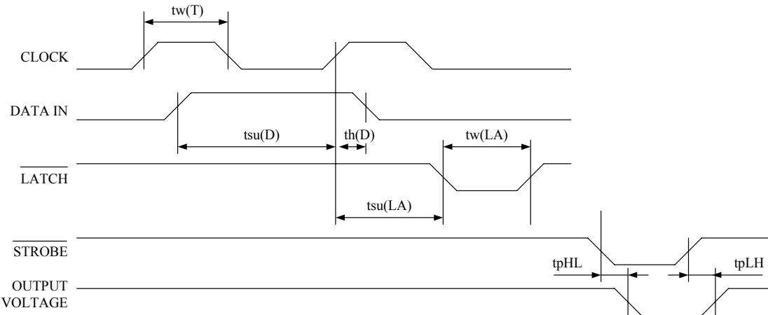
Fig. 2 Thermal Print Head (3T54-2I) Timing Chart
